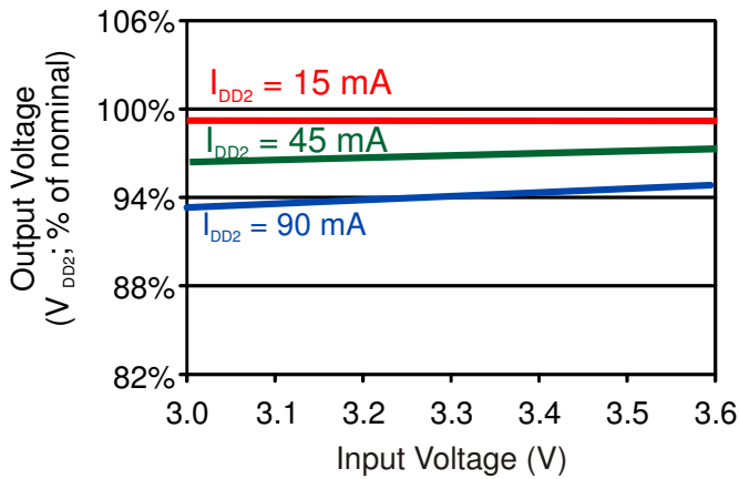
Figure 2. Typical line regulation.
