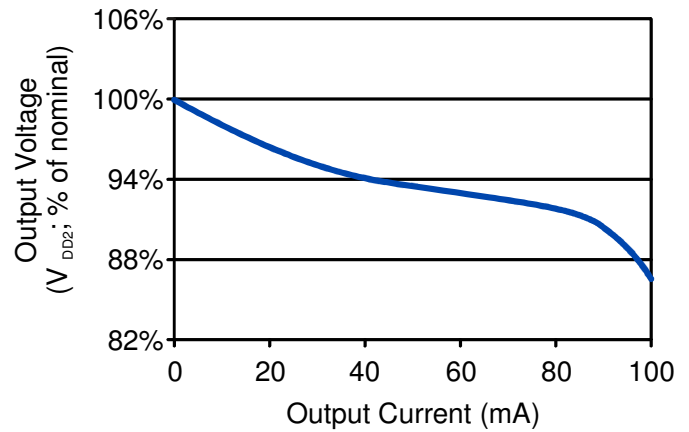
Figure 3. Typical load regulation.
