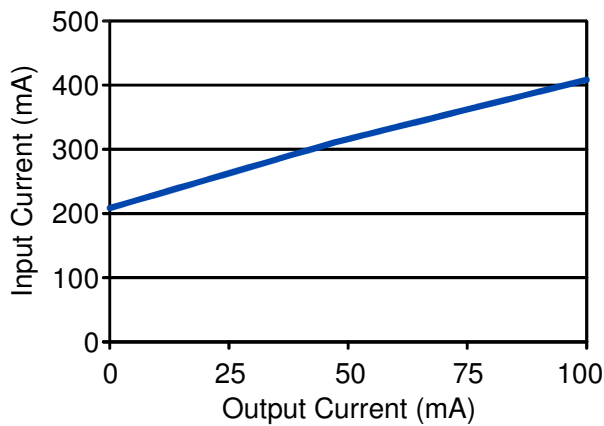
Figure 4. Typical input current versus output current.
