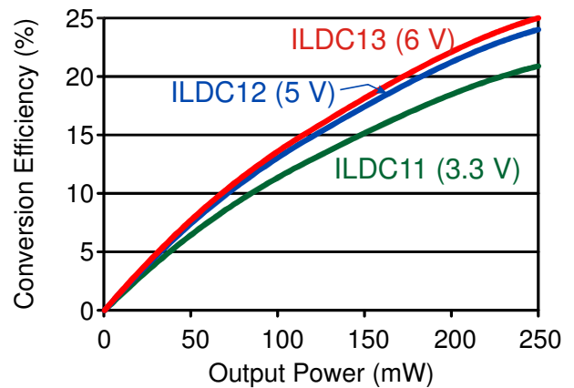
Figure 5. Conversion power efficiency.
