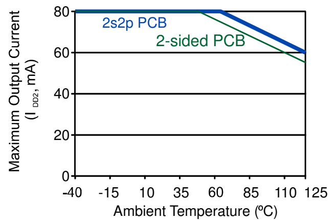
Figure 7. Temperature derating curve (ILDC11).
