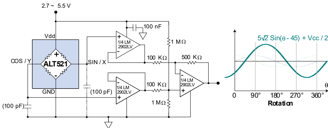
Figure 14. Ultrasensitive rotation counter using a quad Op Amp as a dual-buffered differential amplifier. The gain of the differential amplifier is five, and subtracting the SIN and COS outputs introduces a 45^\circ phase shift and increases the amplitude by a factor of \sqrt{2} .
