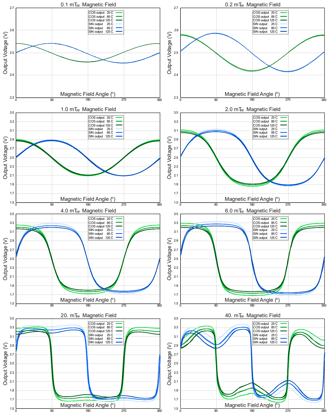
Figure 2. Typical ALT521-10E rotation-mode output at various magnetic fields and temperatures. The supply voltage is 5 V.
