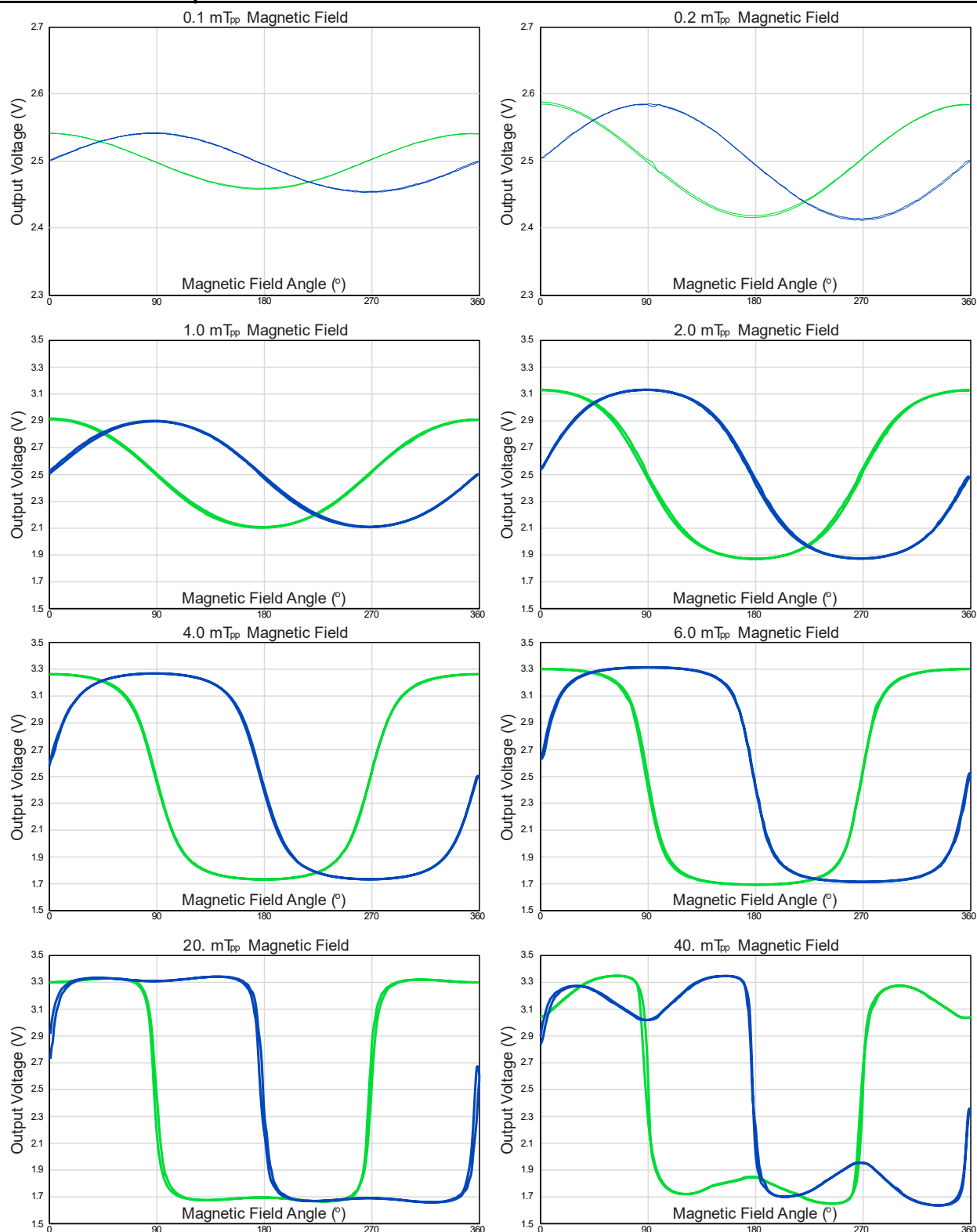
Figure 1. Typical ALT521-10E rotation-mode output at various magnetic fields. The supply voltage is 5 V.
